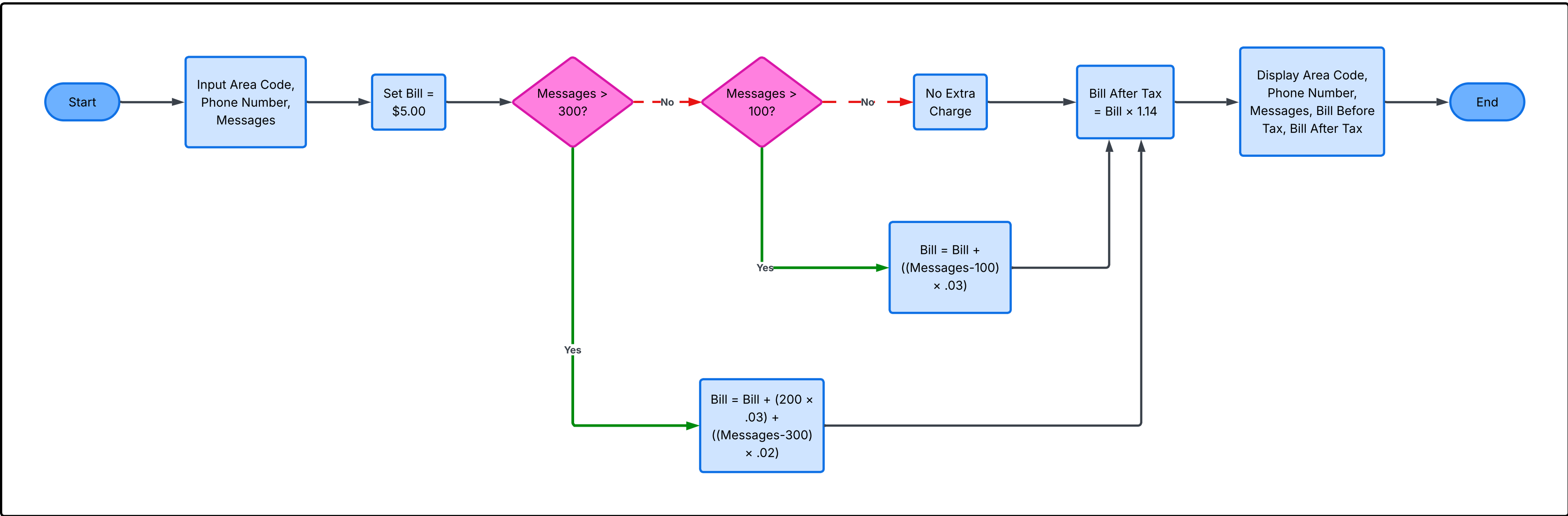
Billing Flowchart
